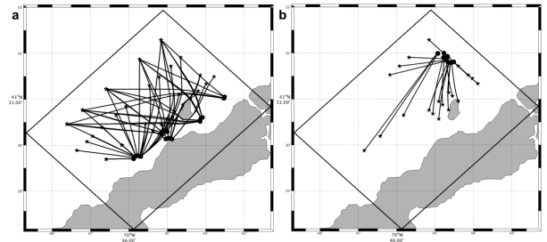
Fig. 6. Candidate time-optimal paths for missions on 21 Oct. 2016: More than 100 paths were computed between several start locations (circles) and targets (stars) spread in the region near Weepeeket islands: (a) Candidates for Mission 1, (b) Candidates for Mission 2
