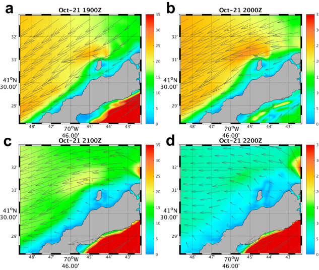
Fig. 5. Ocean current forecasts around Weepeeket Island from the MSEAS PE model : The horizontal currents at 3 m depth are represented by vectors overlaid on a color plot of the flow magnitude (in cm/s). Forecasts are shown at every hour from 19Z to 22Z (3pm EDT to 6pm EDT) during which we completed our sea tests.
